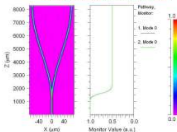
Figure 3.2. Simulation of a 3-dB, 2° Y-branch (a) Designed Y-branch, (b) Performance of the Y-branch
