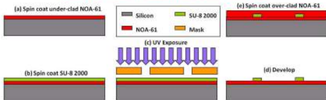
Figure 3.12. Polymer Waveguide Fabrication Process Steps
