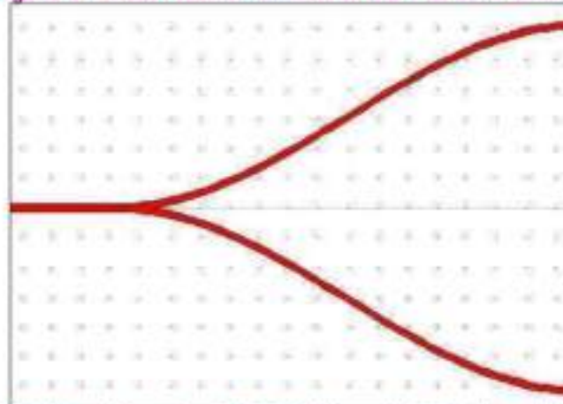
Figure 3.2. Simulation of a 3-dB, 2° Y-branch (a) Designed Y-branch, (b) Performance of the Y-branch
